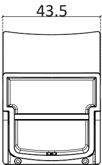
STEP MOUNTED-101
