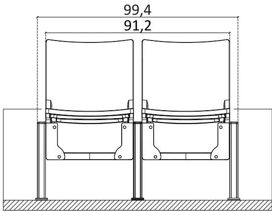
FLOOR MOUNTED-201
